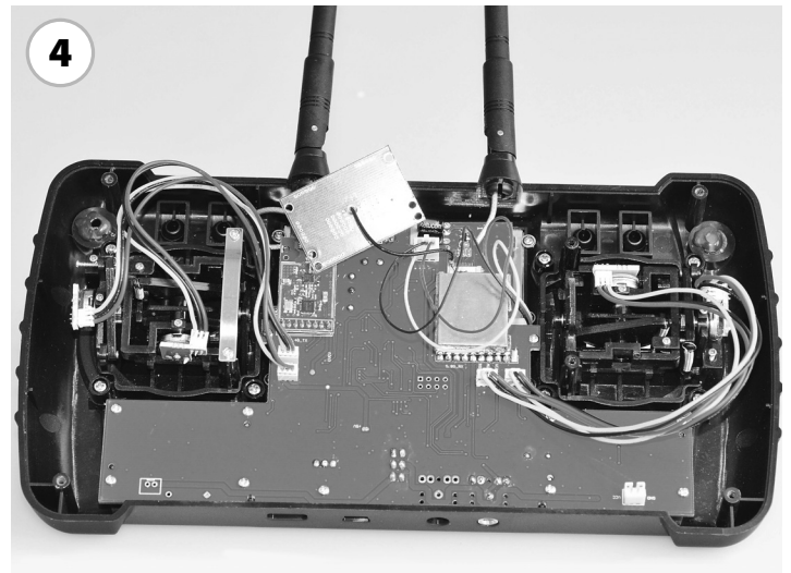
At the end close the cover again with the 4 screws. Pay attention that no cable will be squeezed.
