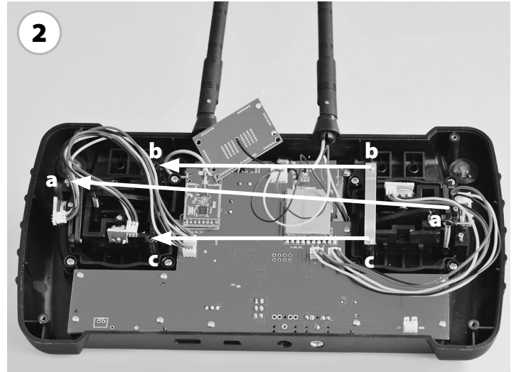
Unscrew a, b and c screws and move screw b, c and the spring to the other side and fix it. Please test afterwards, if the stick is movable smooth or not.
